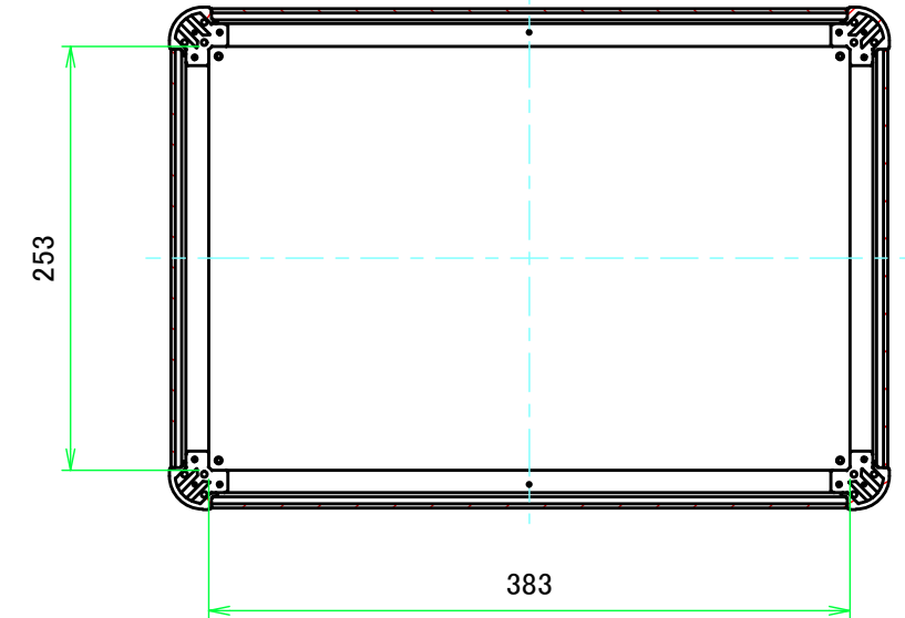
C-C (1:5)
